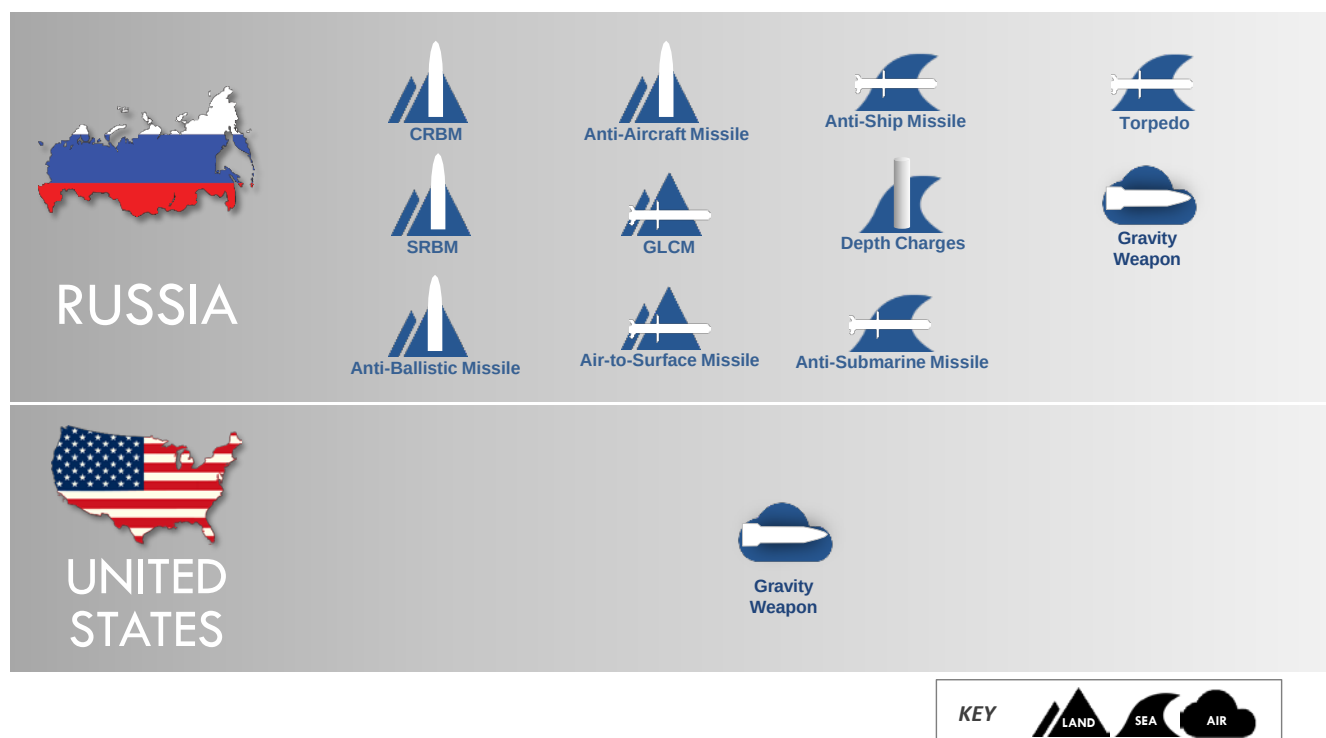
Figure 4. Russia's Non-Strategic Nuclear Challenge
